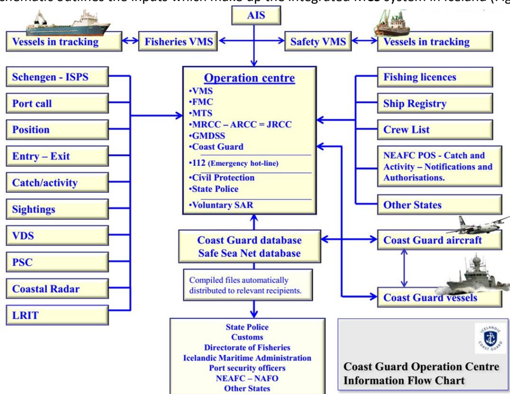
Figure 5. Schematic outlining the inputs which make up the integrated Monitoring, Control and Surveillance (MCS) system in Iceland.
