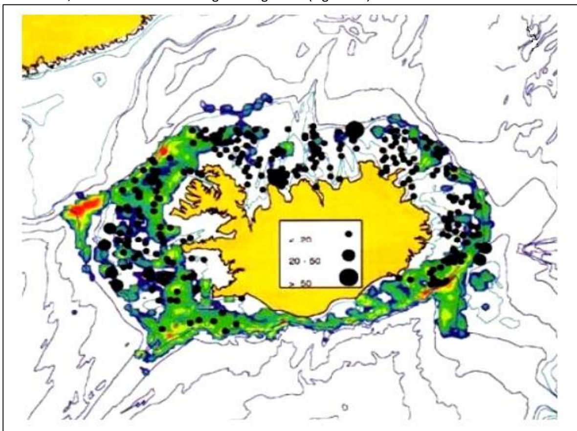
Figure 26. Biomass of sponge bycatch in 2002, superimposed on fishing effort as mean annual swept area ( \text{nm}^2 per 1^\circ latitude x 1^\circ longitude cell). Black dots indicate total biomass (kg/h otter trawl haul) of sponges in the 2002 groundfish survey by the Marine Research Institute. Source:
