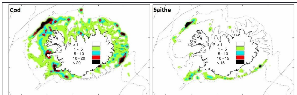
Figure 12. Cod (left) and saithe (right) fishing grounds in 2014. Dark areas indicate highest catch (tonnes/nmi 2 ).
