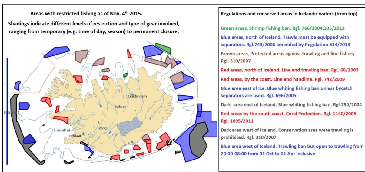
Figure 5. All closures according to the Fisheries directorate by November 2015 26 .
