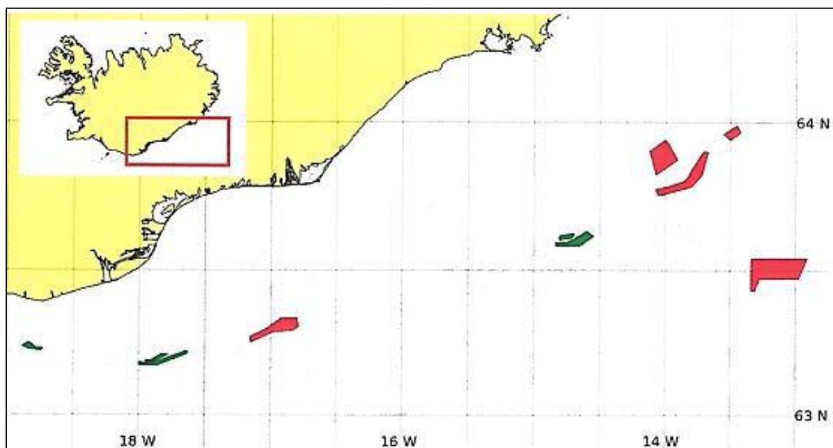
Figure 27. Location of closed areas for the protection of cold water corals in water to the southeast of Iceland.
