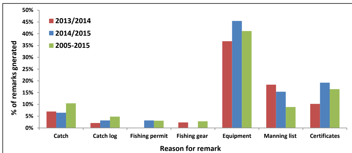
Figure 6. Reasons for the generation of remarks during Coast Guard inspections during the 2013-2014 (Red) and 2014-2015 (Blue) fishing seasons and the period from 1 st January 2005 to 31 st August 2015 (Green).
